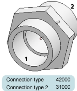
GF_239105_SLEEVE_NIPPLE_M_R
