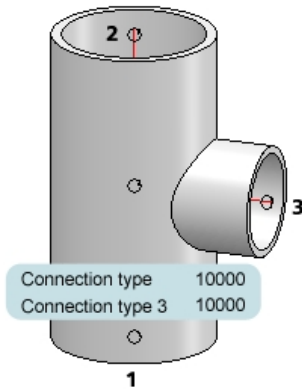
EN10253-4-A_TEE_RED
